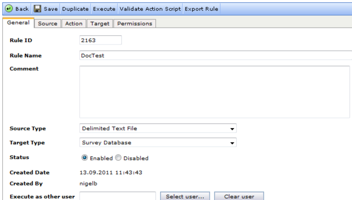
Figure 53 The Current Rule > General tab showing the Execute as other user option
