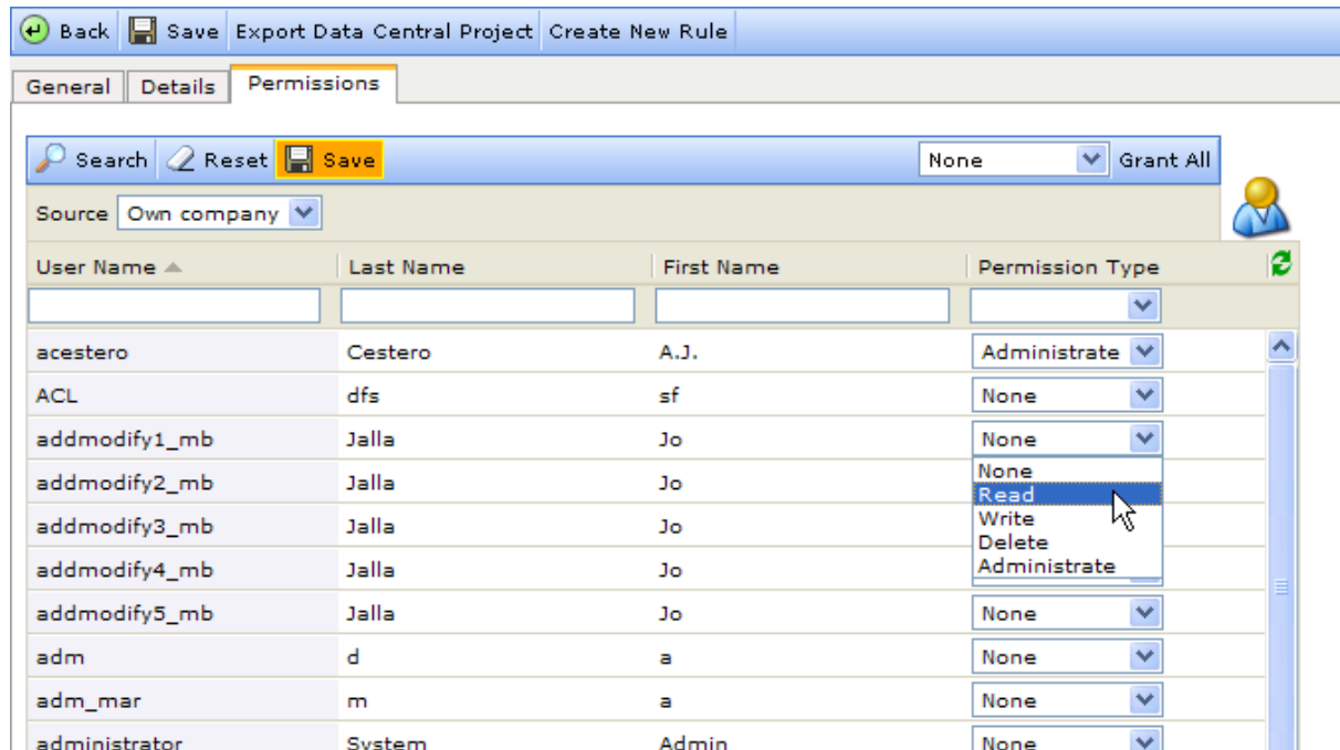
Figure 89 Example of the Permissions tab
