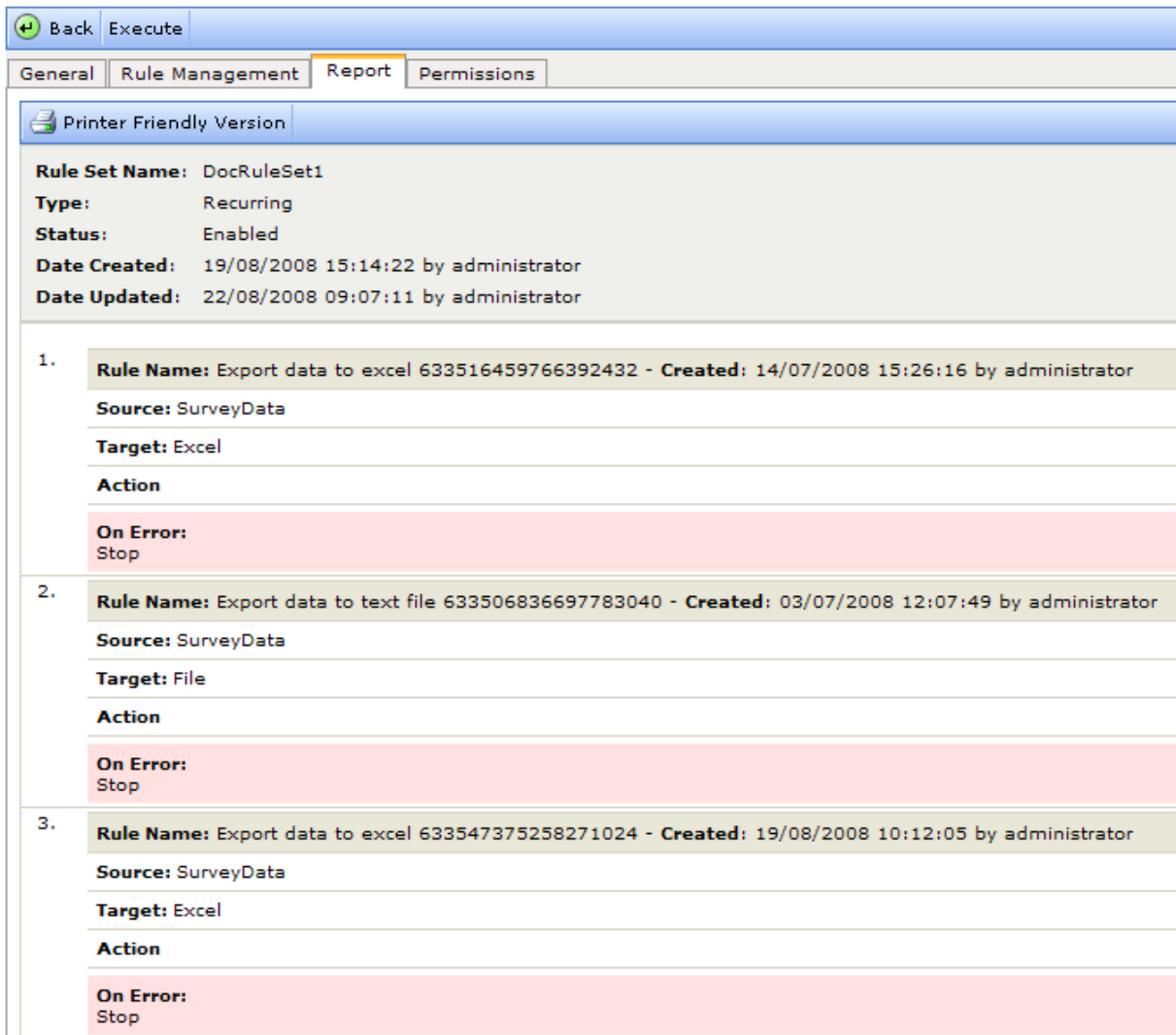
Figure 79 Example of the Report tab
