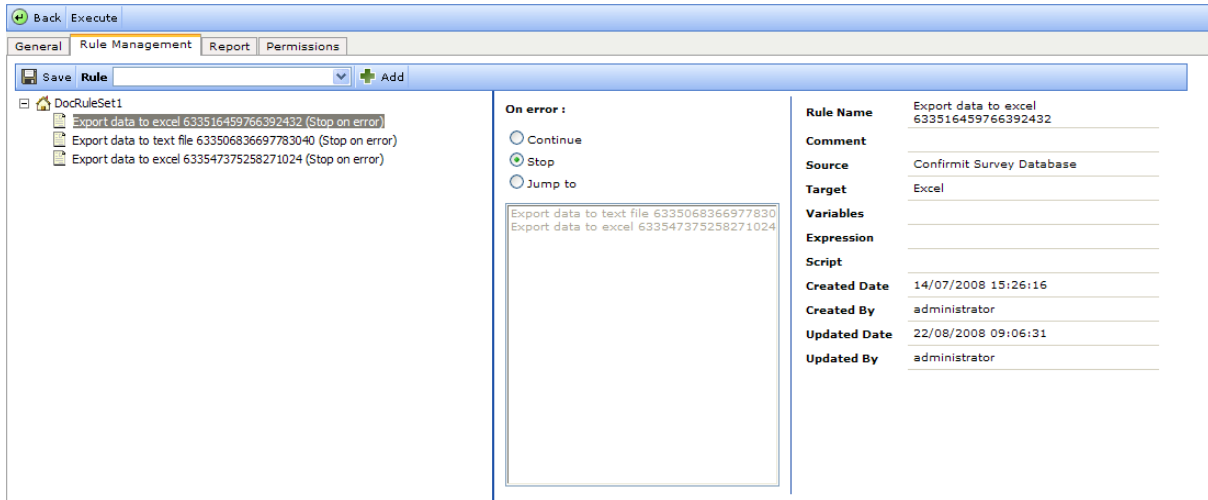
Figure 76 Example of the Rule Management tab
