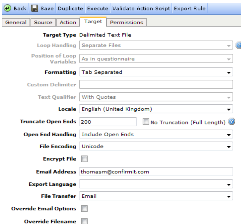
Figure 63 The Target tab when Delimited Text File is selected
