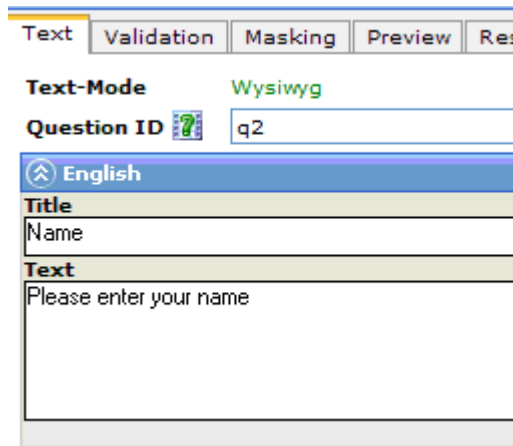
Figure 59 Example of an Open Text question
