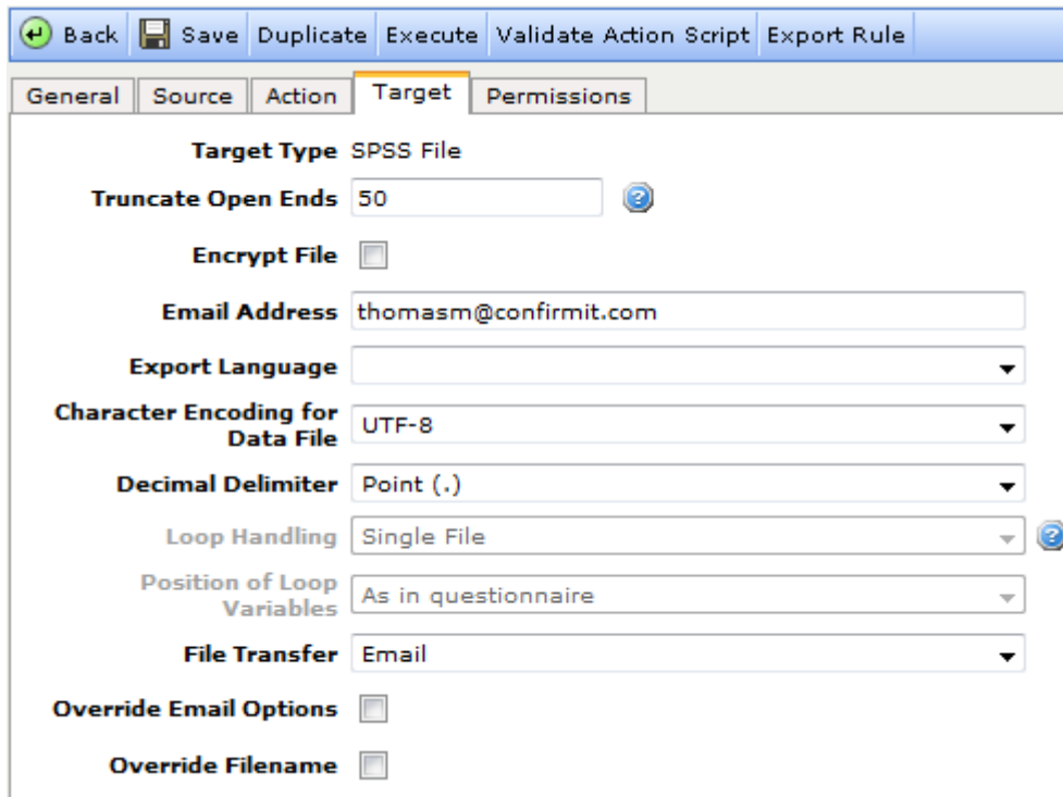
Figure 68 The Target tab when SPSS is selected
