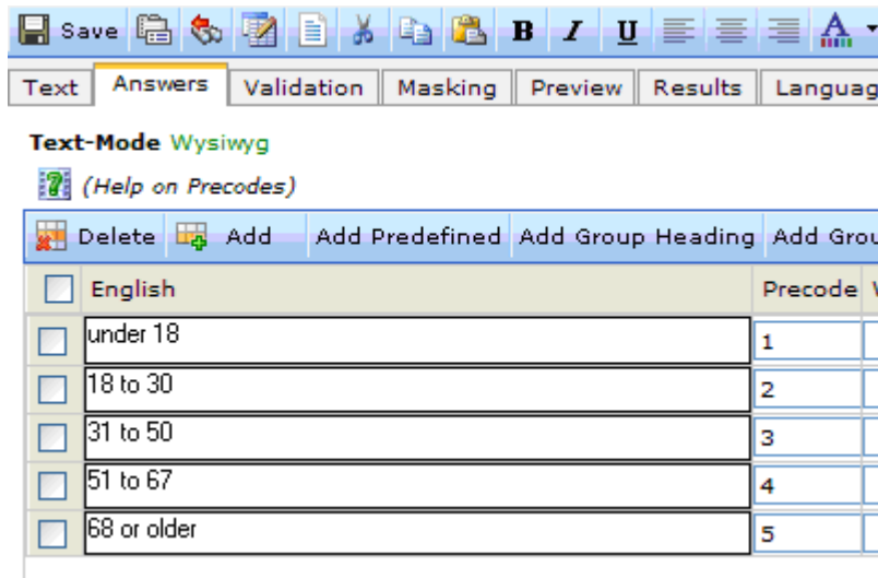
Figure 60 The q4 answer options
