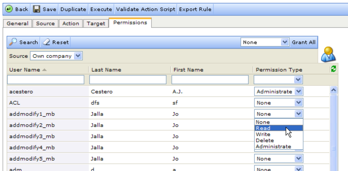
Figure 73 Example of the Permissions tab for a rule
