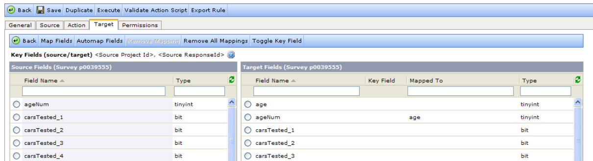
Figure 72 The age field from the Source is mapped to the ageNum field in the Target
